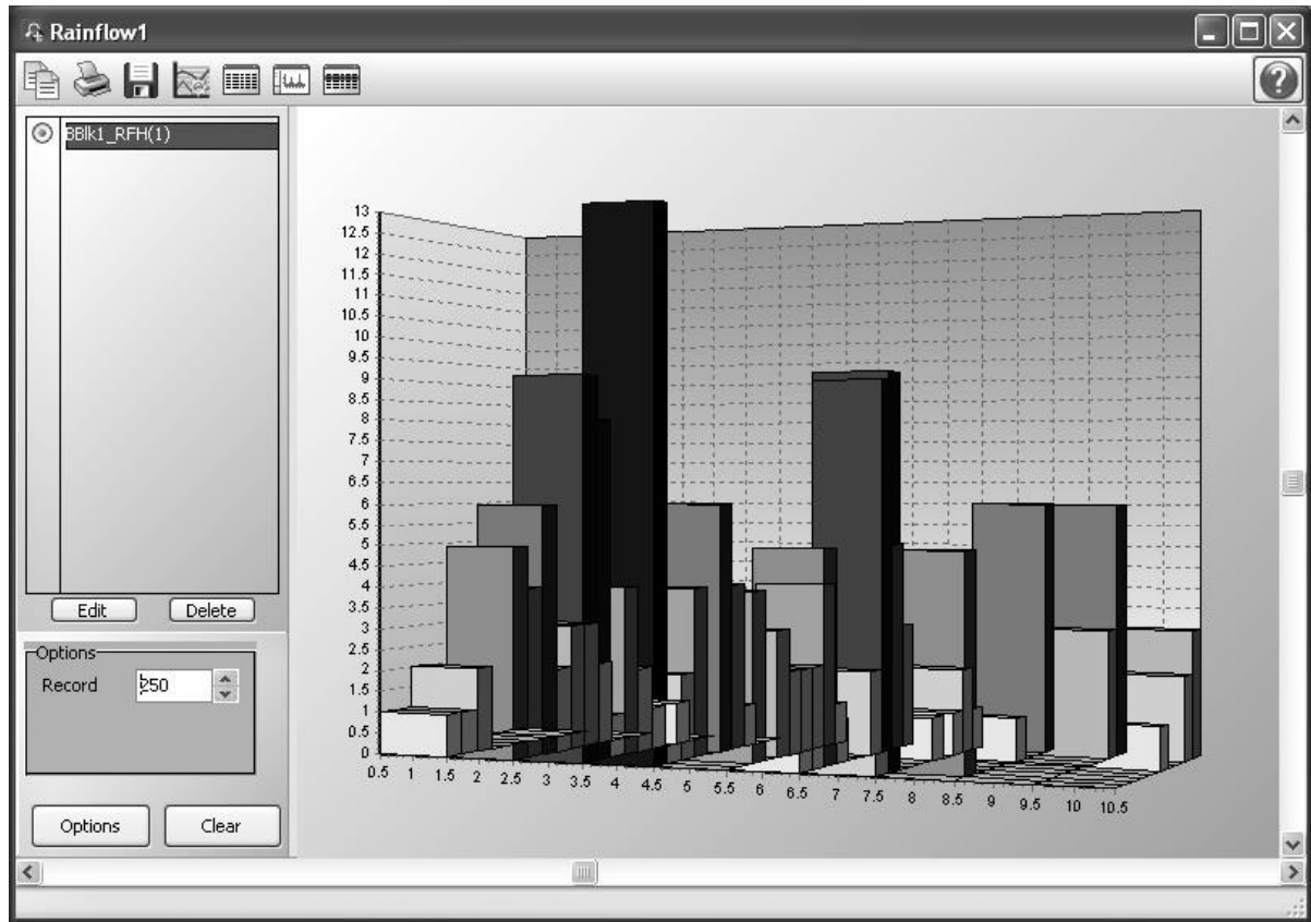
FIGURE 6.5-6. Rainflow Histogram
