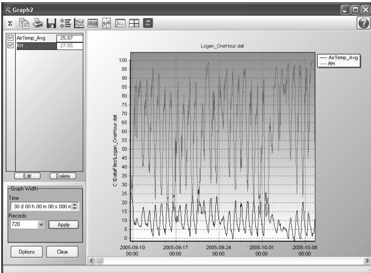
FIGURE 6.5-1. Line Graph
