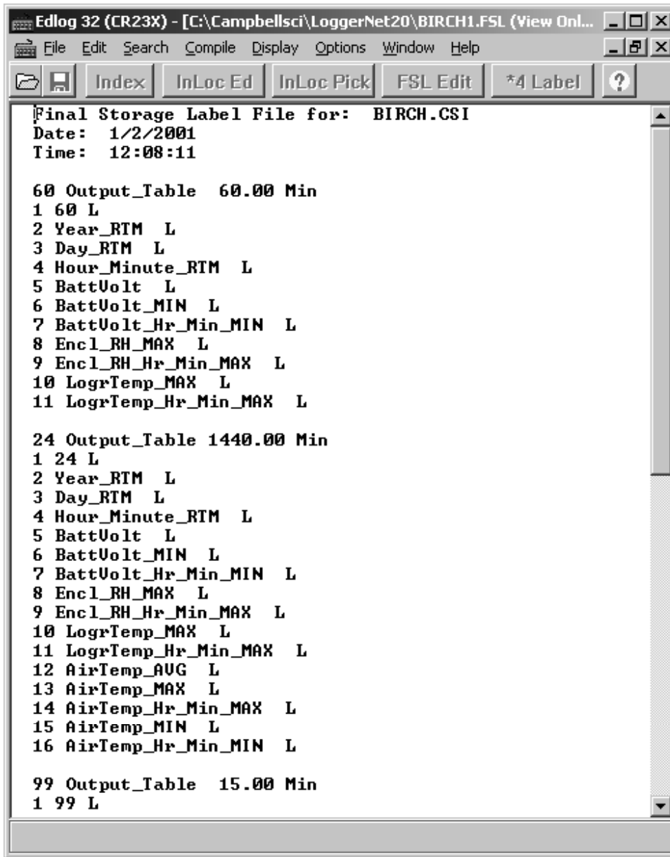
FIGURE 8.2-2. FSL file
