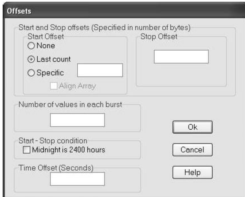
FIGURE 8.2-9. Offsets options
