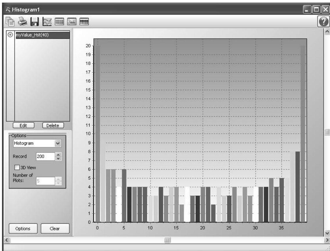
FIGURE 6.5-3. Histogram
