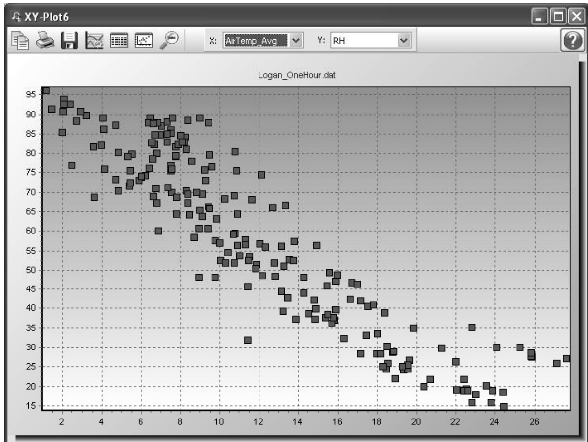
FIGURE 6.5-5. XY Plot
