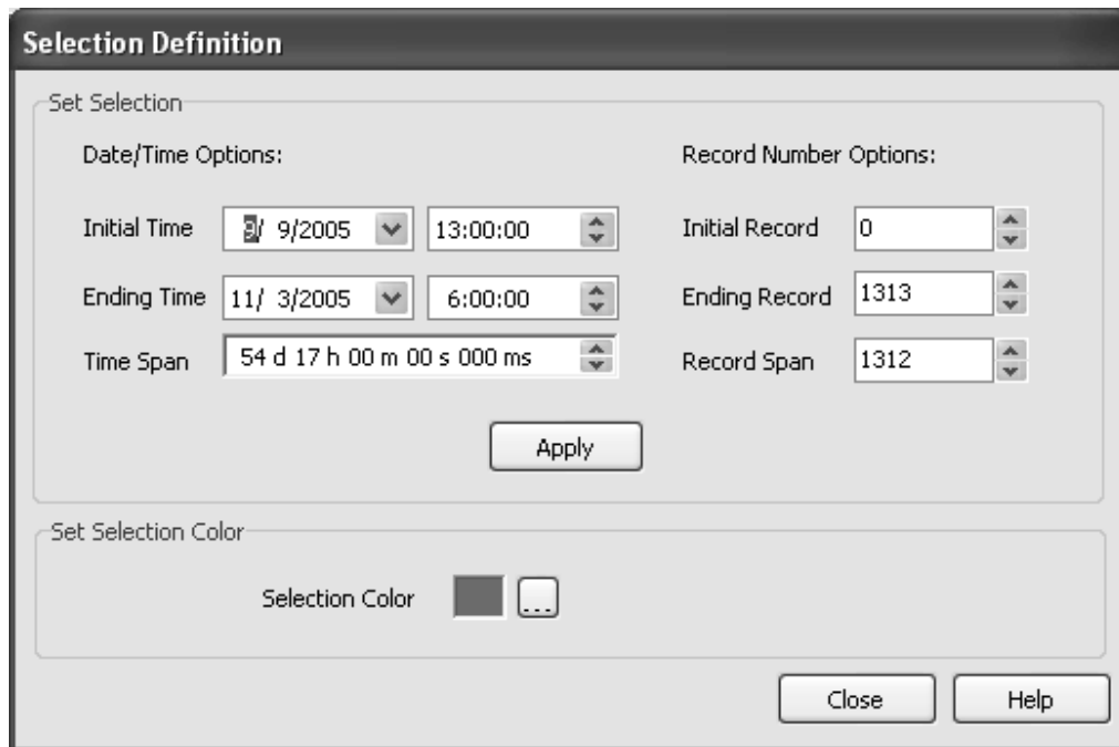
FIGURE 6.6-1. Selection Definition
