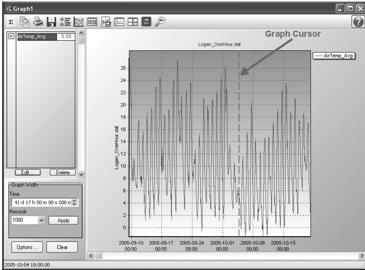
FIGURE 6.5-2. Graph Cursor
